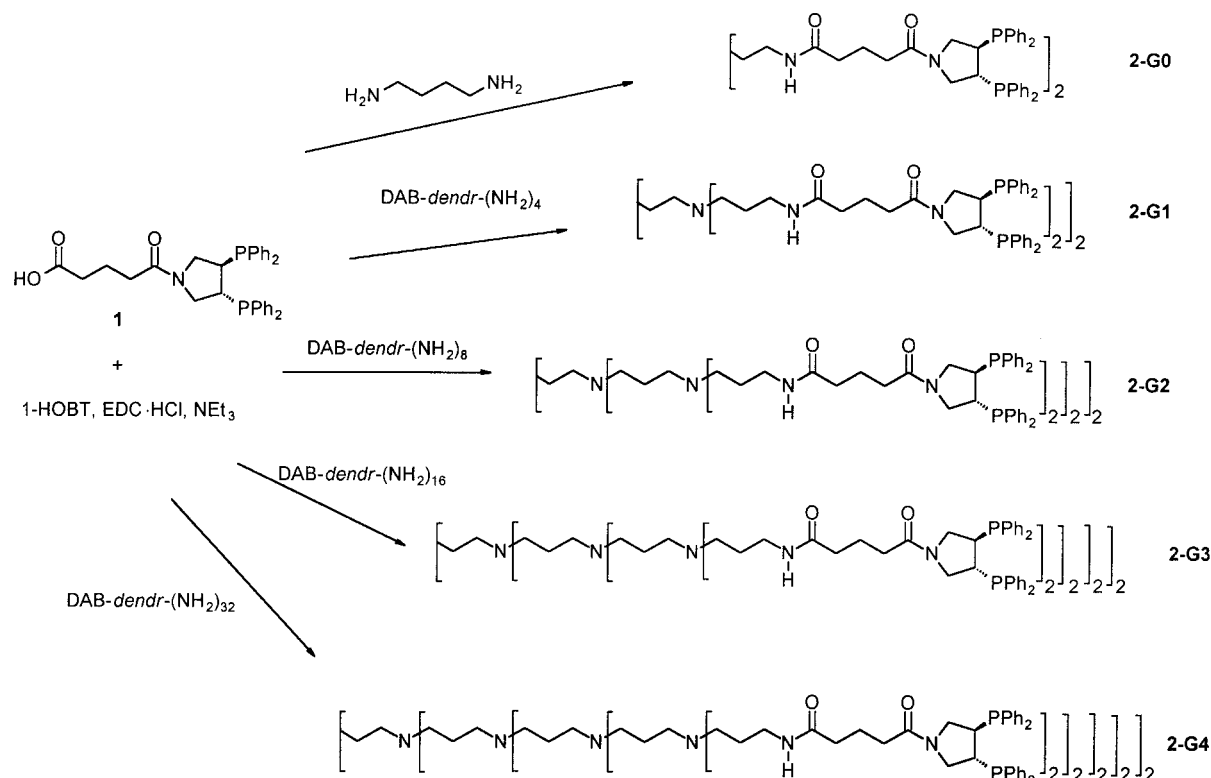
Scheme 1. Coupling of the chiral phosphine carboxylate 1 with the amino end groups of the poly(propyleneimine) dendrimers of generations 0–4 (DAB=1,4-diaminobutane).
