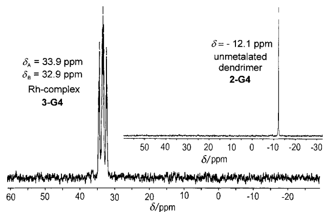
Figure 3. ^{31}\text{P} NMR spectrum of the fourth-generation rhododendrimer 3-G4 showing the complete metalation of the phosphine binding sites.
