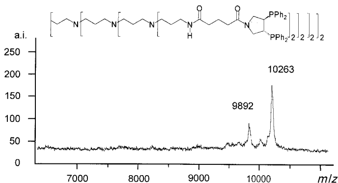
Figure 2. MALDI-TOF mass spectrum of the third-generation phosphine-functionalized dendrimer 2-G3 .
