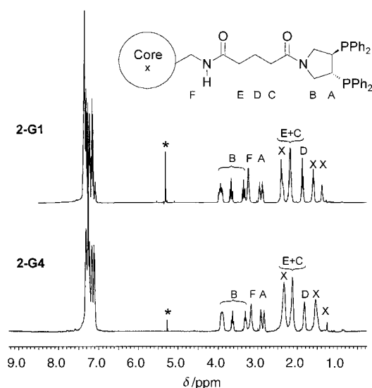
Figure 1. Comparison of the 500 MHz ^1\text{H} NMR spectra of 2-G0 and 2-G4 demonstrating the similarity in the resonance patterns (* = \text{CH}_2\text{Cl}_2 ).
