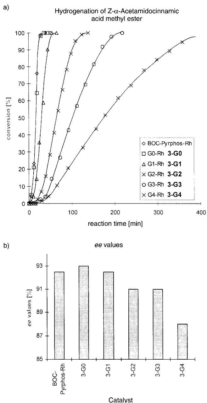
Figure 4. a) Conversion curves of the asymmetric hydrogenation of Z -methyl- \alpha -acetamidocinnamate for the different catalyst generations. b) Enantioselectivity of the asymmetric hydrogenation of Z -methyl- \alpha -acetamidocinnamate for the different catalyst generations.
