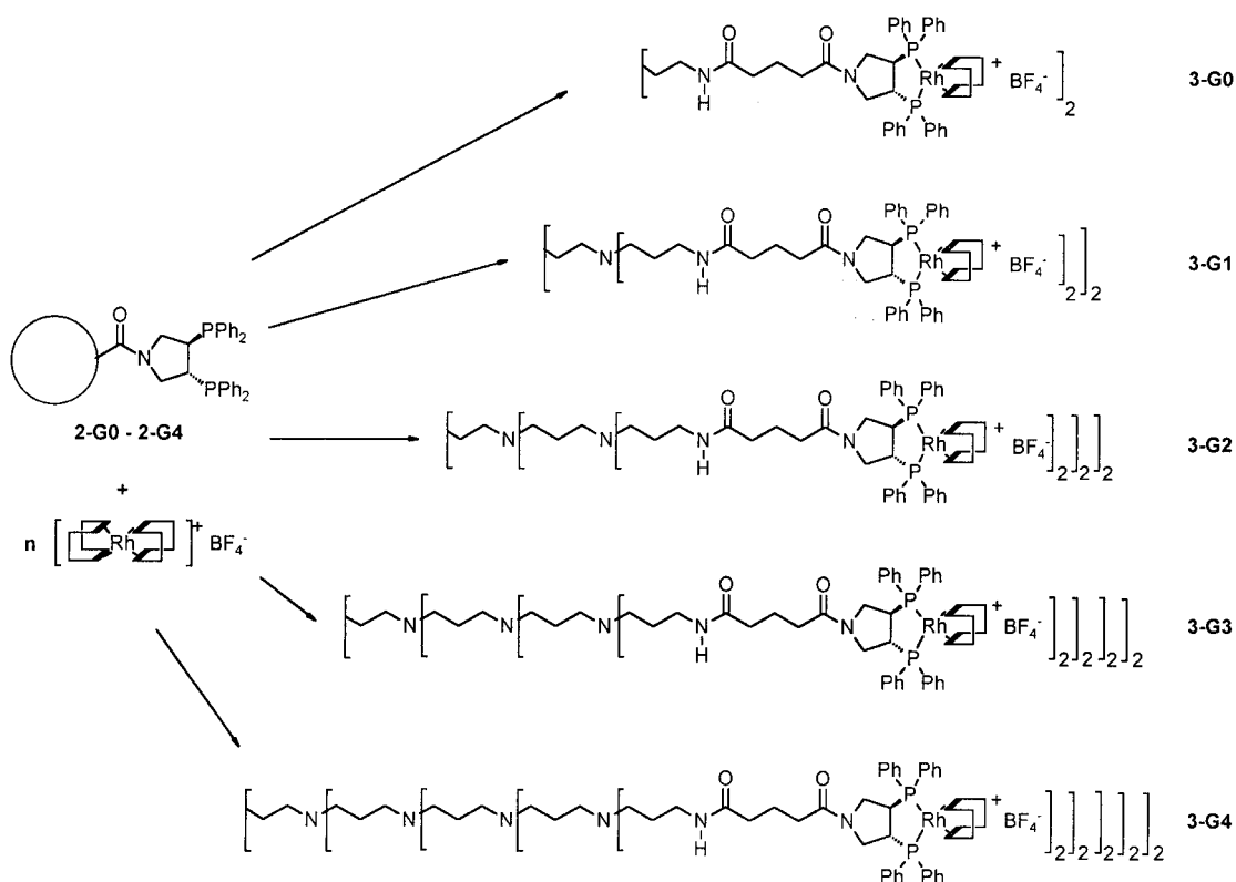
Scheme 2. Synthesis of the metallodendrimers 3-G0–3-G4 by reaction of 2-G0–2-G4 with [\text{Rh}(\text{cod})_2]\text{BF}_4 .
