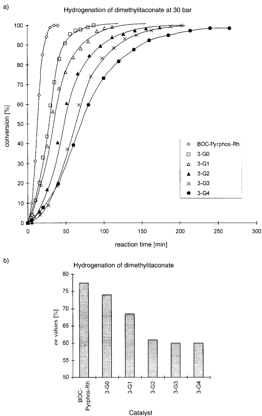
Figure 5. a) Conversion curves of the asymmetric hydrogenation of dimethyl itaconate for the different catalyst generations. b) Enantioselectivity of the asymmetric hydrogenation of dimethyl itaconate for the different catalyst generations.
